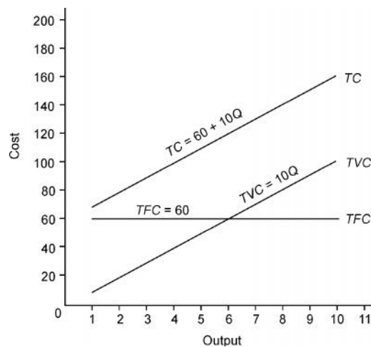
Fig. 3.9 Linear Cost Functions
