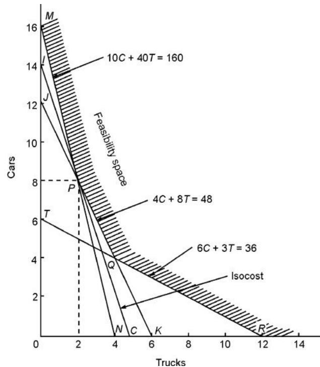
Fig. 3.16 Cost-Minimisation: Graphical Solution
